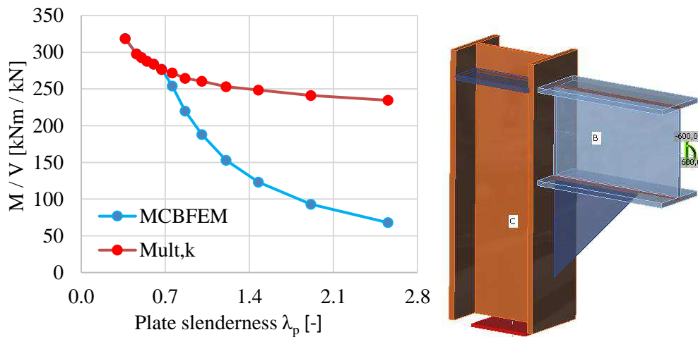
The influence of plate slenderness on the resistance of portal frame joint with slender stiffener
