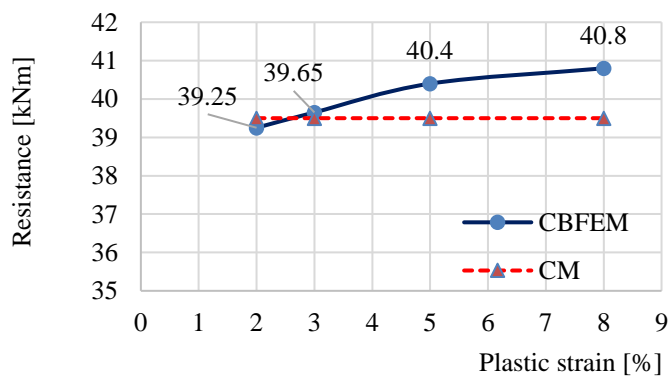
Influence of the limit value of plastic strain on the moment resistance
