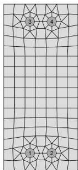
Mesh on end plate, with 7 elements on width
