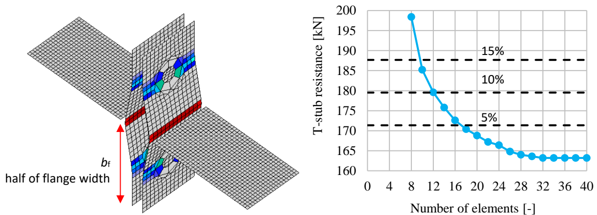
Influence of number of elements on the T-stub resistance
