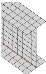
Mesh on beam with constrains between web and flange plate
