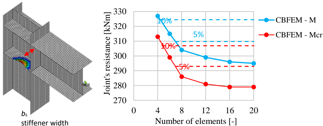
First buckling mode and influence of number of elements along the stiffener on the moment resistance
